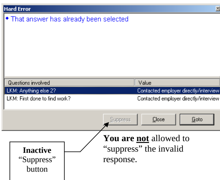
Figure C4a. Hard Error Message
